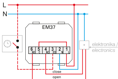
motorni pogon (ograničena uporaba s podnim grijanjem) / motor drive (limited use with underfloor heating)
