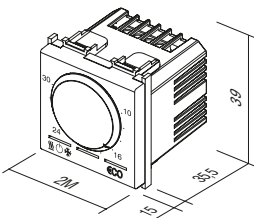
motorni pogon (ograničena uporaba s podnim grijanjem) / motor drive (limited use with underfloor heating)
