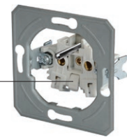
BV Steckklemmen BV plug-in contacts
